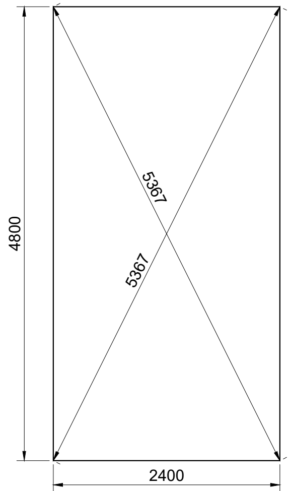
Camping Pod 2.4x4.8 with terrace FLOOR FRAME
