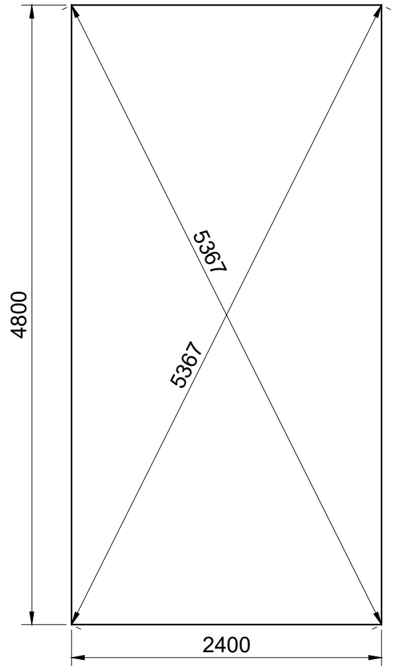
Camping Pod 2.4x4.8 FLOOR FRAME
