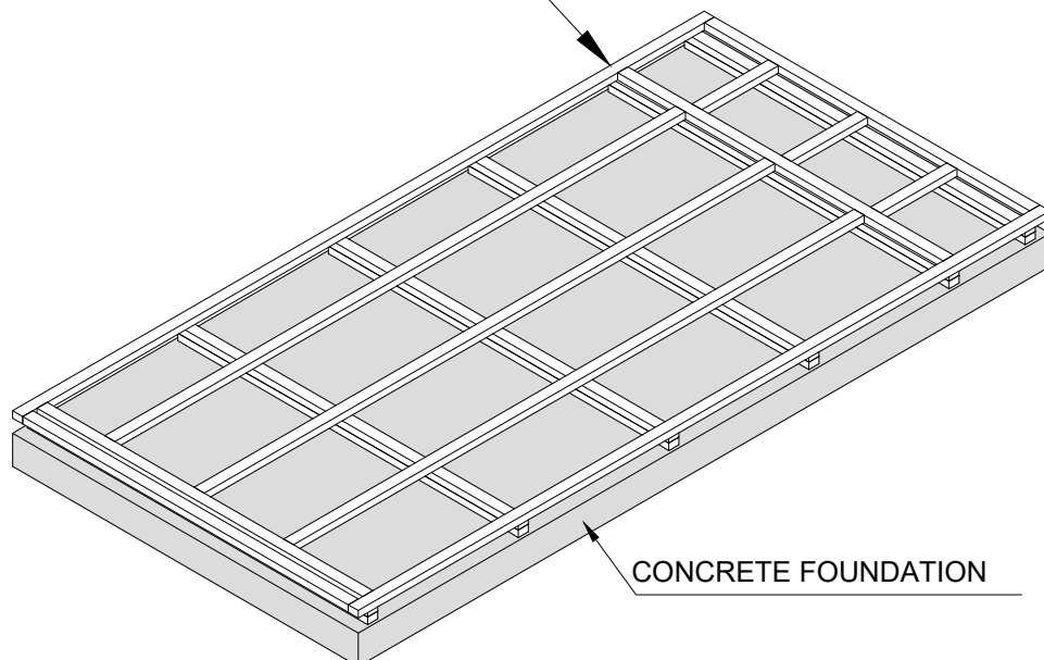
Camping Pod 2.4x4.8 with terrace FLOOR FRAME
