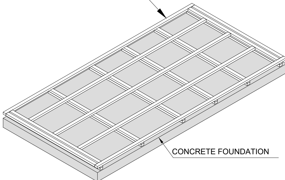
Camping Pod 2.4x4.8 FLOOR FRAME
