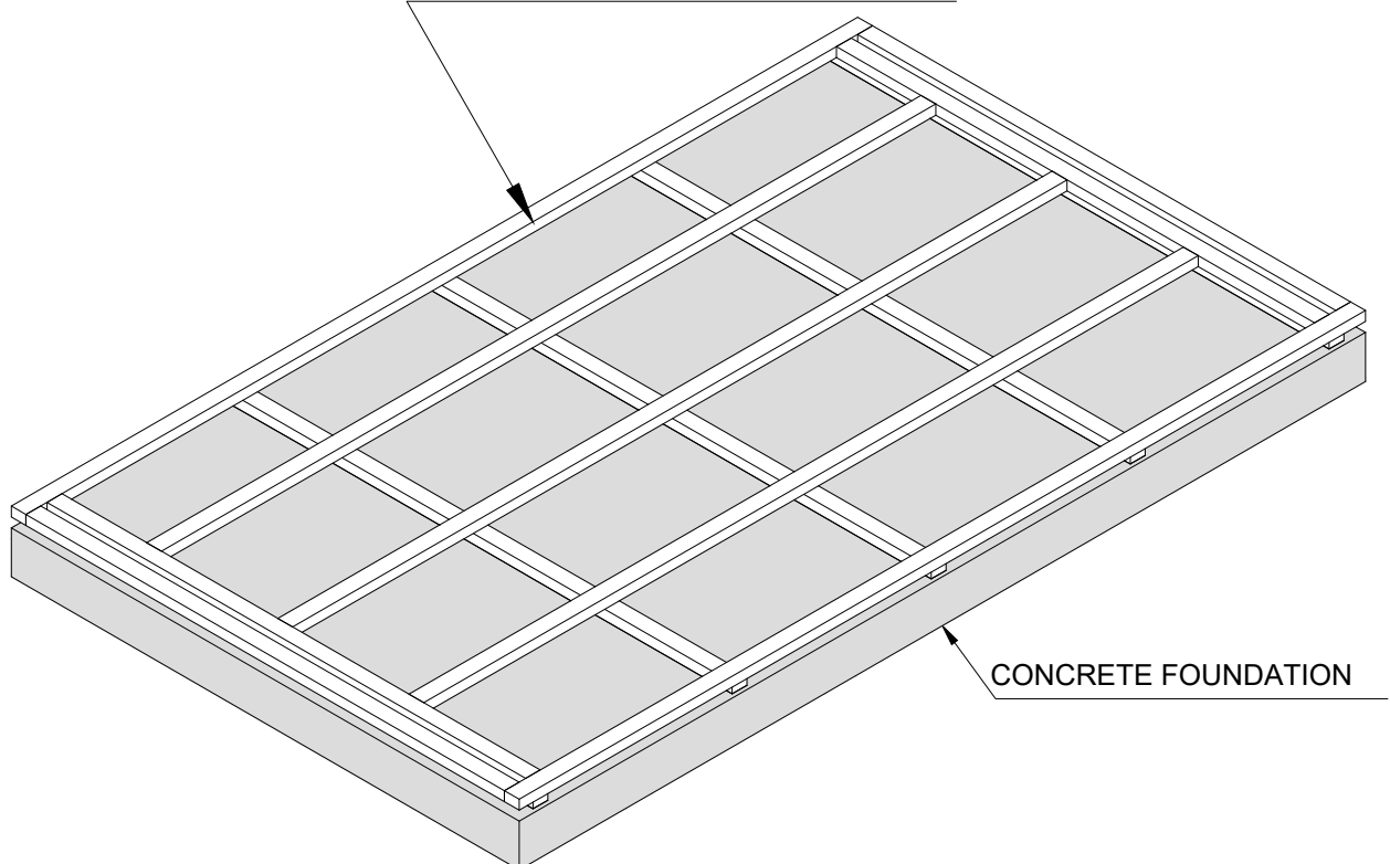
Camping Pod 2.4x4 FLOOR FRAME
