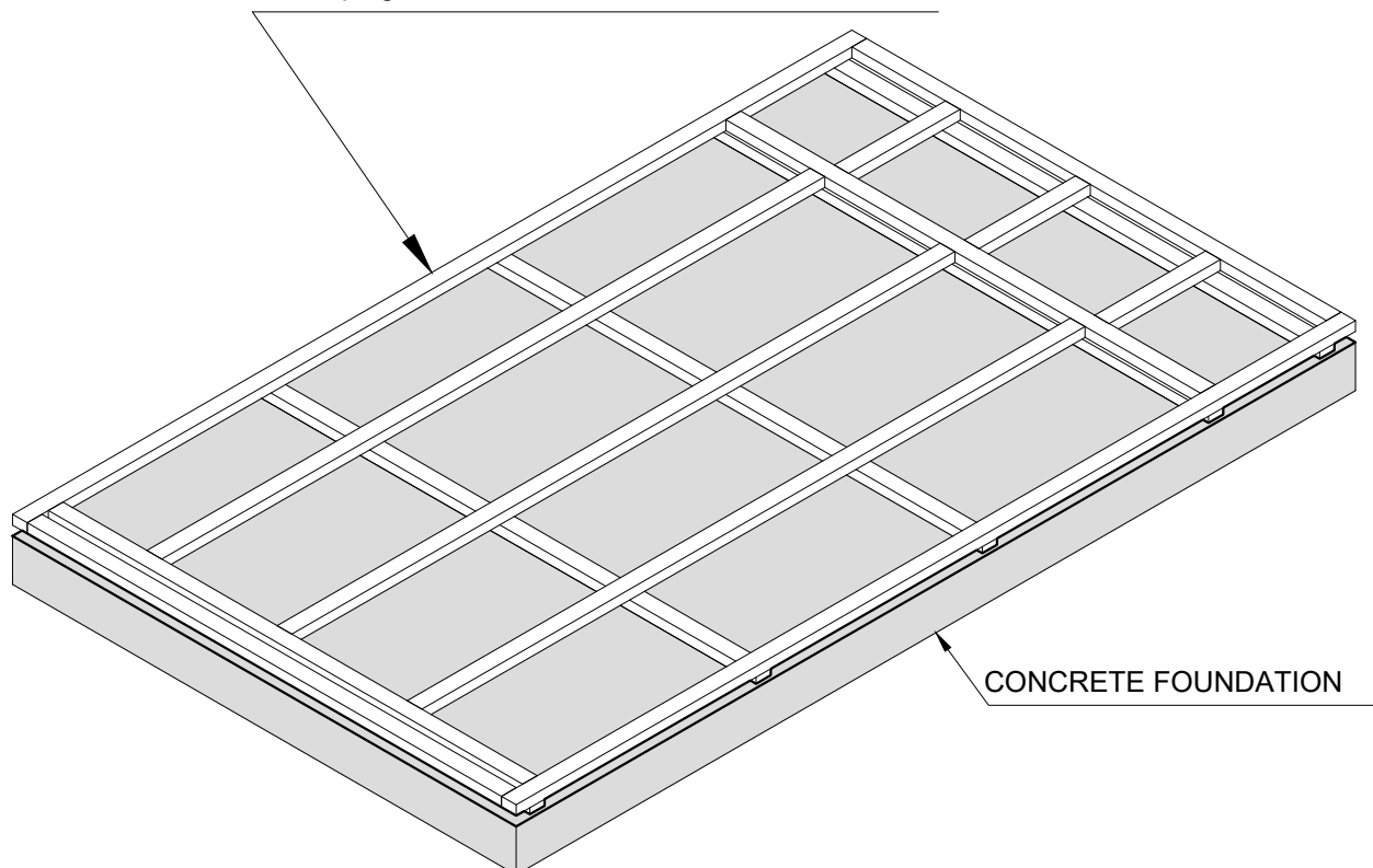
Camping Pod 2.4x4 with terrace FLOOR FRAME
