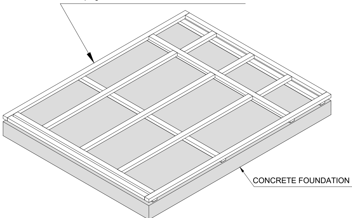
Camping Pod 2.4x3 with terrace FLOOR FRAME
