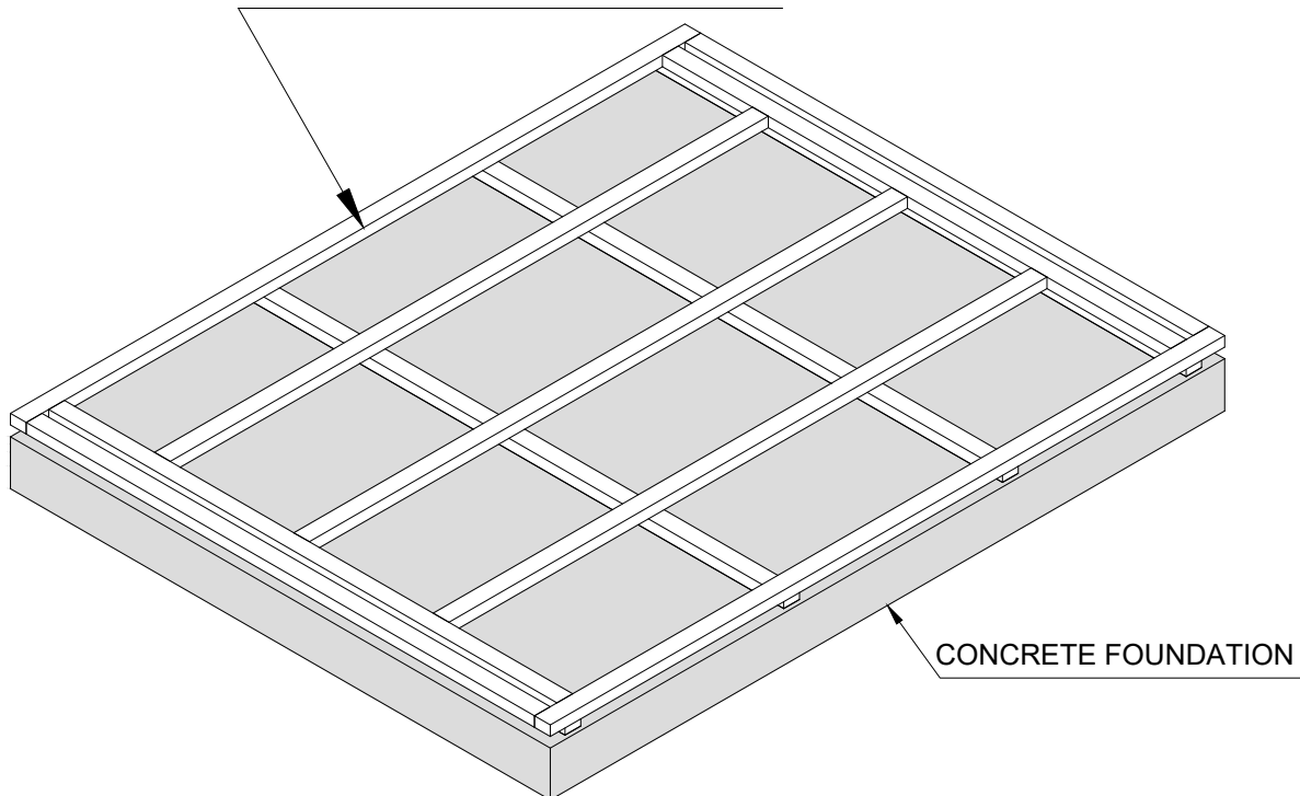
Camping Pod 2.4x3 FLOOR FRAME
